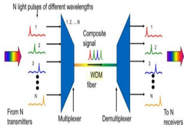
Fig1: WDM Network Architecture
